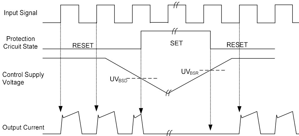
Fig.6 Under-Voltage Protection (Low-side)
