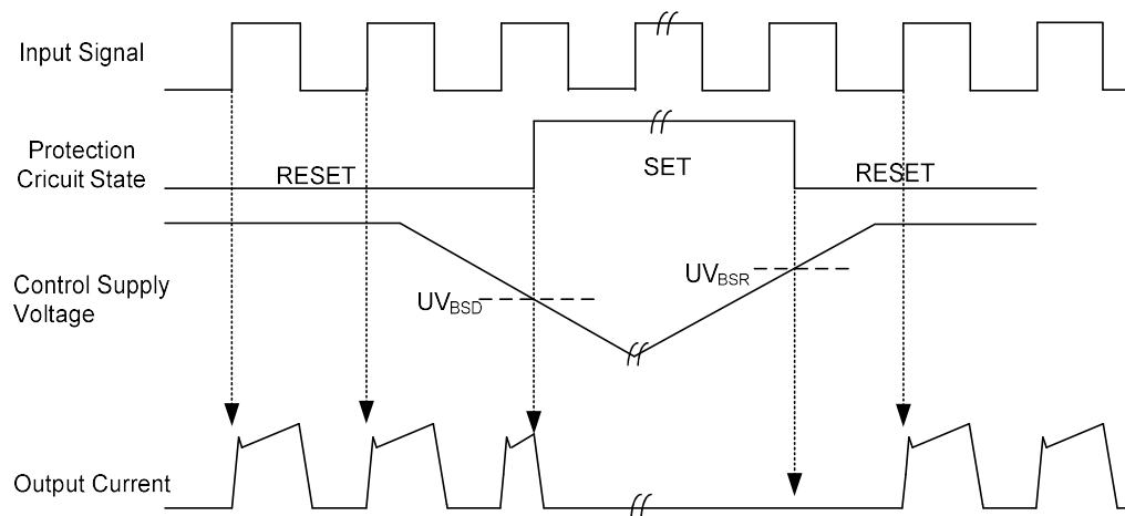
Fig.6 Under-Voltage Protection (Low-side)
