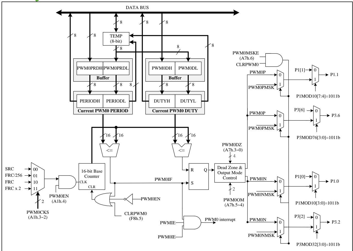
PWM0 Structure
