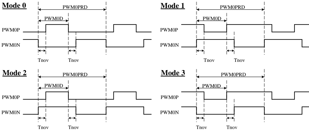
PWM0 normal mode output mode
