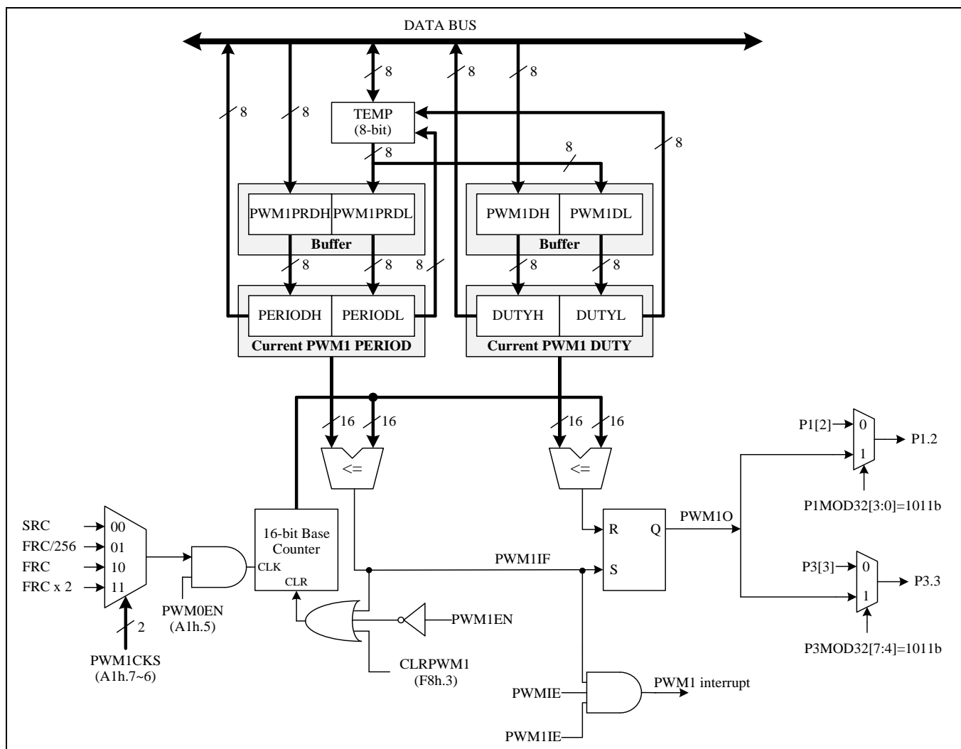
PWM1 structure
